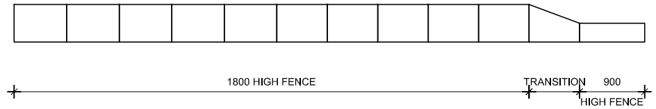
TYPICAL SIDE FENCE ELEVATION
